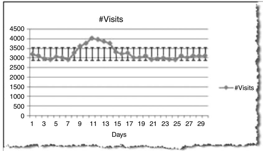
FIGURE 3.9 Standard deviation
